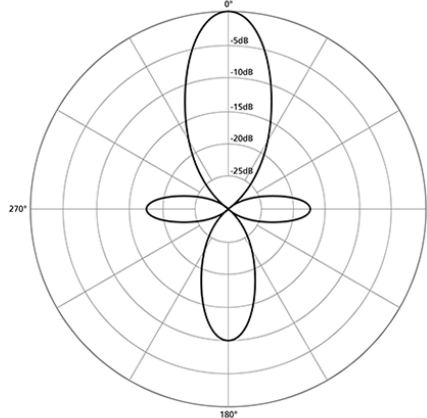
Shotgun
