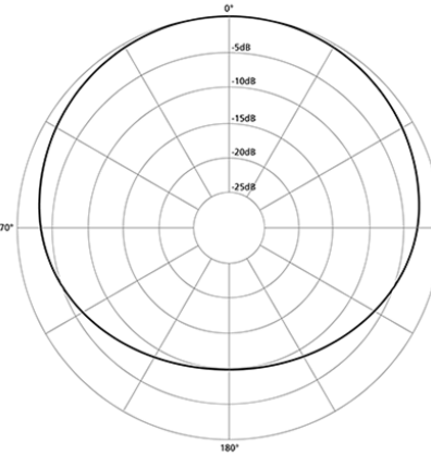
Subcardioid
