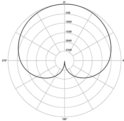
Cardioid
