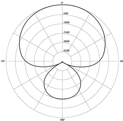
Supercardioid
