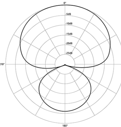
Hypercardioid
